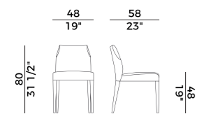
772 sedia \ chair
